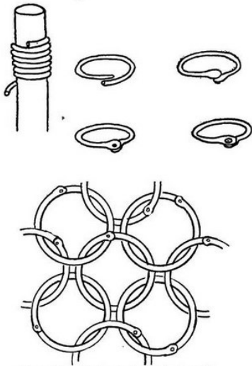
FIG. 18. Method of making mail.
